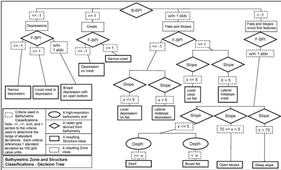
Figure 9. A flowchart of the decisions made by the algorithms that derive zone and structure classes from broad scale bathymetric position index (B-BPI), fine scale BPI (F-BPI), slope and depth.
