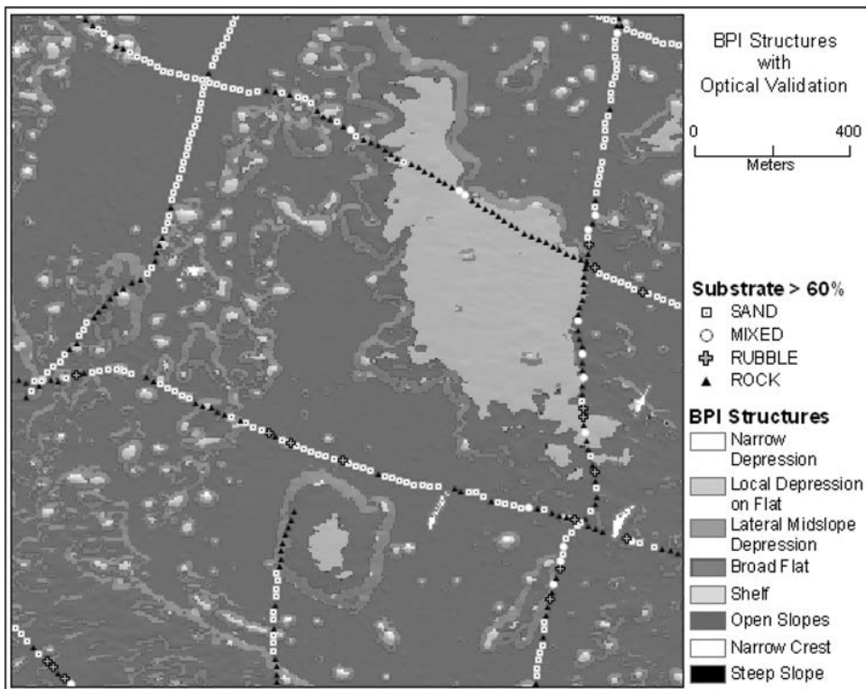
Figure 12. BPI Structures overlaid with optical validation. This is a sample from the Saipan anchorage data set that was surveyed by CRED in 2003 and 2004. The structures were derived from a bathymetric grid (5-m pixel size), and the optical validation represents interpretations of videos from a towed underwater video camera-sled. A qualitative assessment validates a pattern of associations between substrates and BPI structures.
