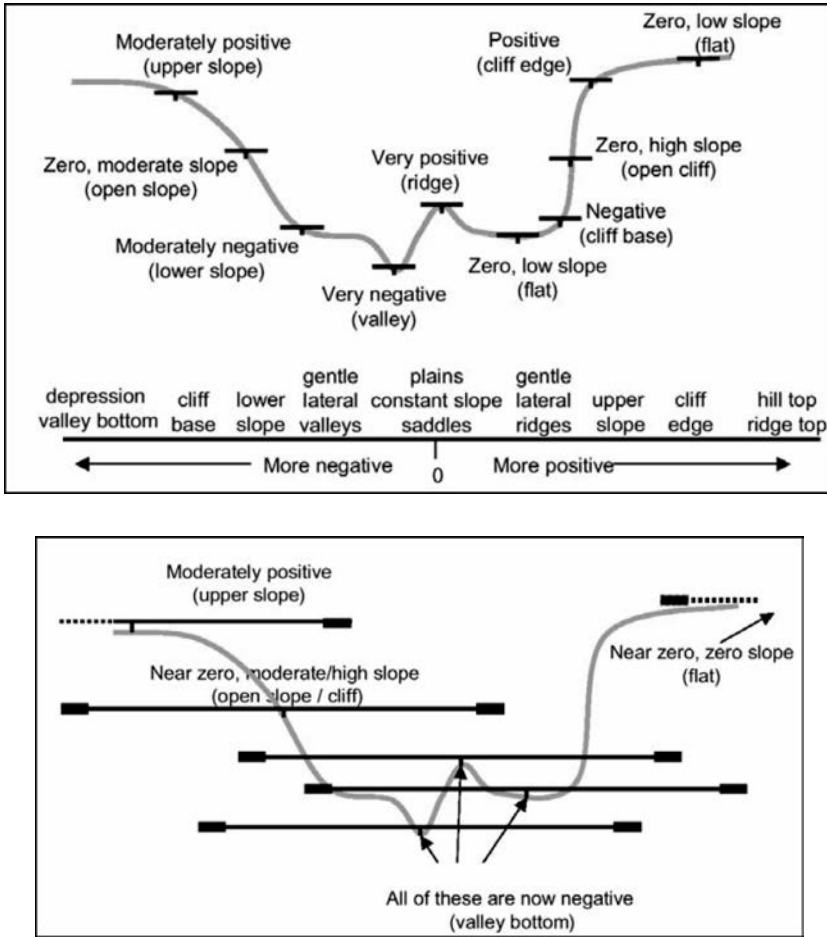
Figure 4. A description of the resulting bathymetric position index (BPI) values that are derived from bathymetry. These are based on a topographic position index by Weiss (2001). Top describes fine scale BPI values. Bottom describes broad scale BPI values. (Courtesy of Weiss 2001.)
