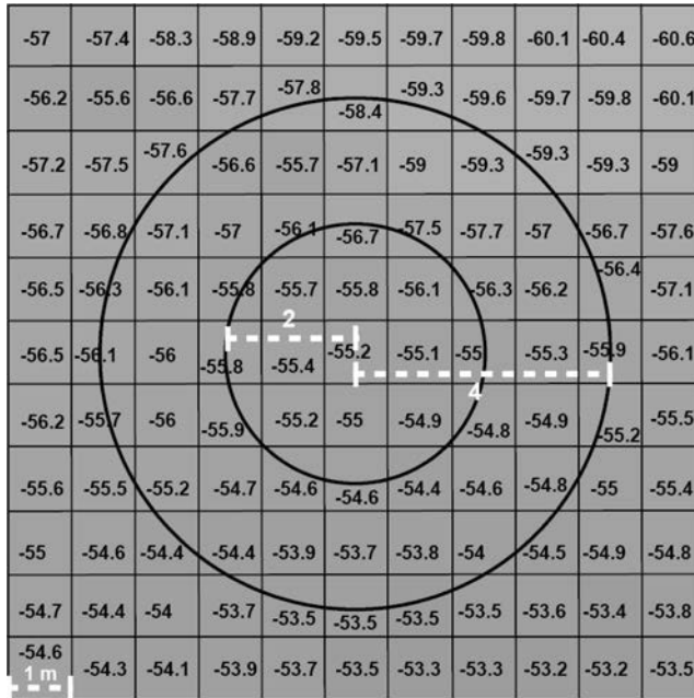
Figure 3. Example of the variables used to derive bathymetric position index (BPI) from bathymetry. The grid cells here (1 m resolution) represent bathymetry as negative values. The annulus has an outer radius of 4 and an inner radius of 2. Therefore the BPI scalefactor is 4 (outer radius multiplied by bathymetry resolution).
