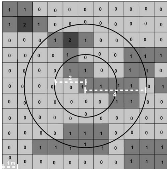
Figure 5. Example of the variables used to derive bathymetric position index (BPI) from bathymetry. The grid cells represent a derived BPI grid. Negative values are lower than their neighbors. Positive values are higher than their neighbors. Values of zero are flat areas or areas with constant slope.
