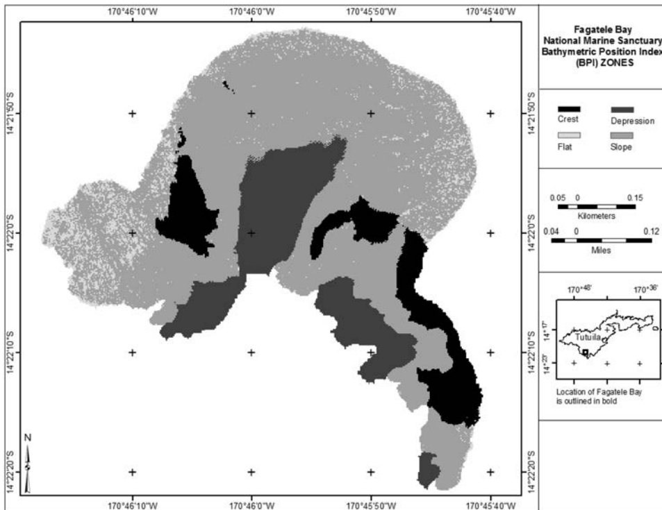
Figure 10. BPI Zones for Fagatele Bay National Marine Sanctuary.
